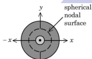
Figure 1. electron probability density for 2s orbital
