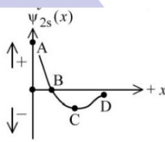
Figure 2. wave function for 2s orbital
